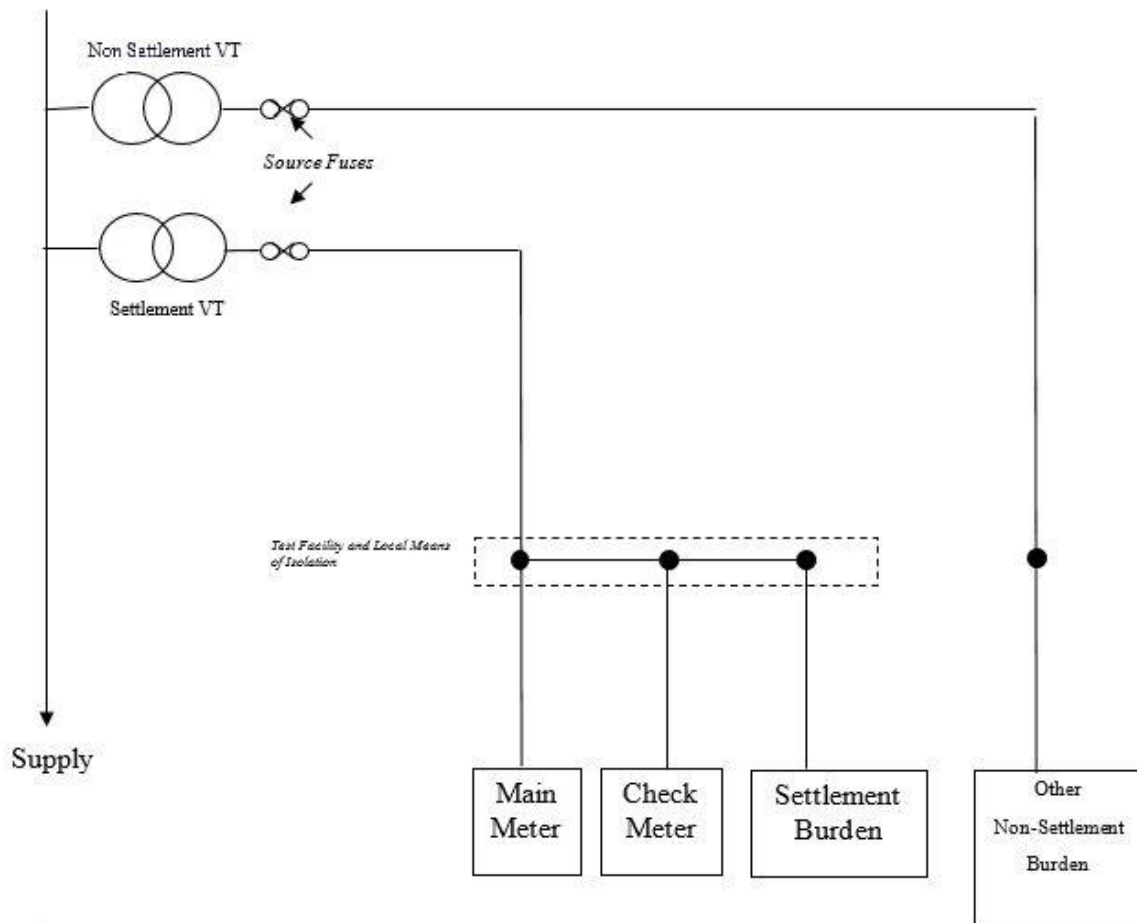
Figure 1: Fusing arrangements for cable runs of less than 30 metres distance between source fusing and local means of isolation 16 17 .
