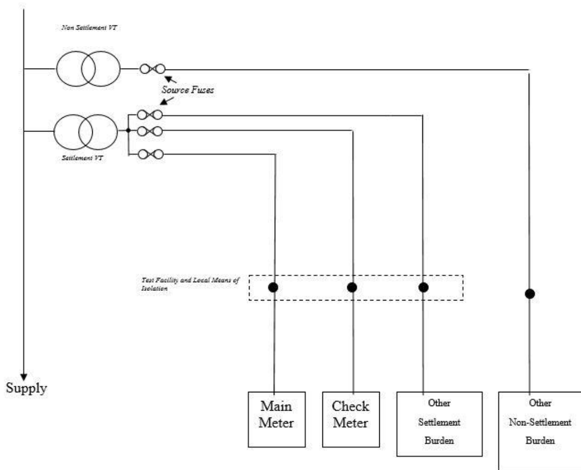
Figure 2: Fusing arrangements for cable runs of more than 30 metres distance between source fusing and local means of isolation 18 19 .
